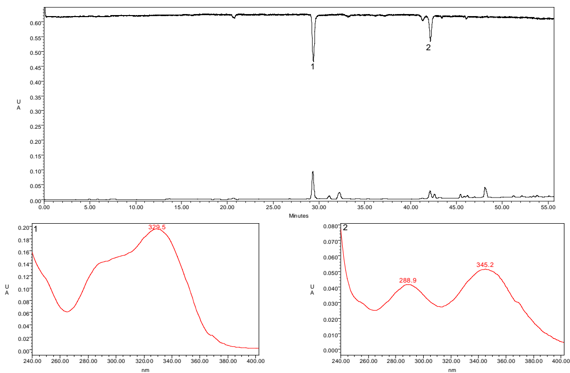
Figure 8. HPLC profile of the ethyl ester fraction of the ethyl acetate extract of M. australis . Numbered peaks contained active antioxidant compounds; the bottom chart shows the UV absorption profile of the numbered active peaks.
